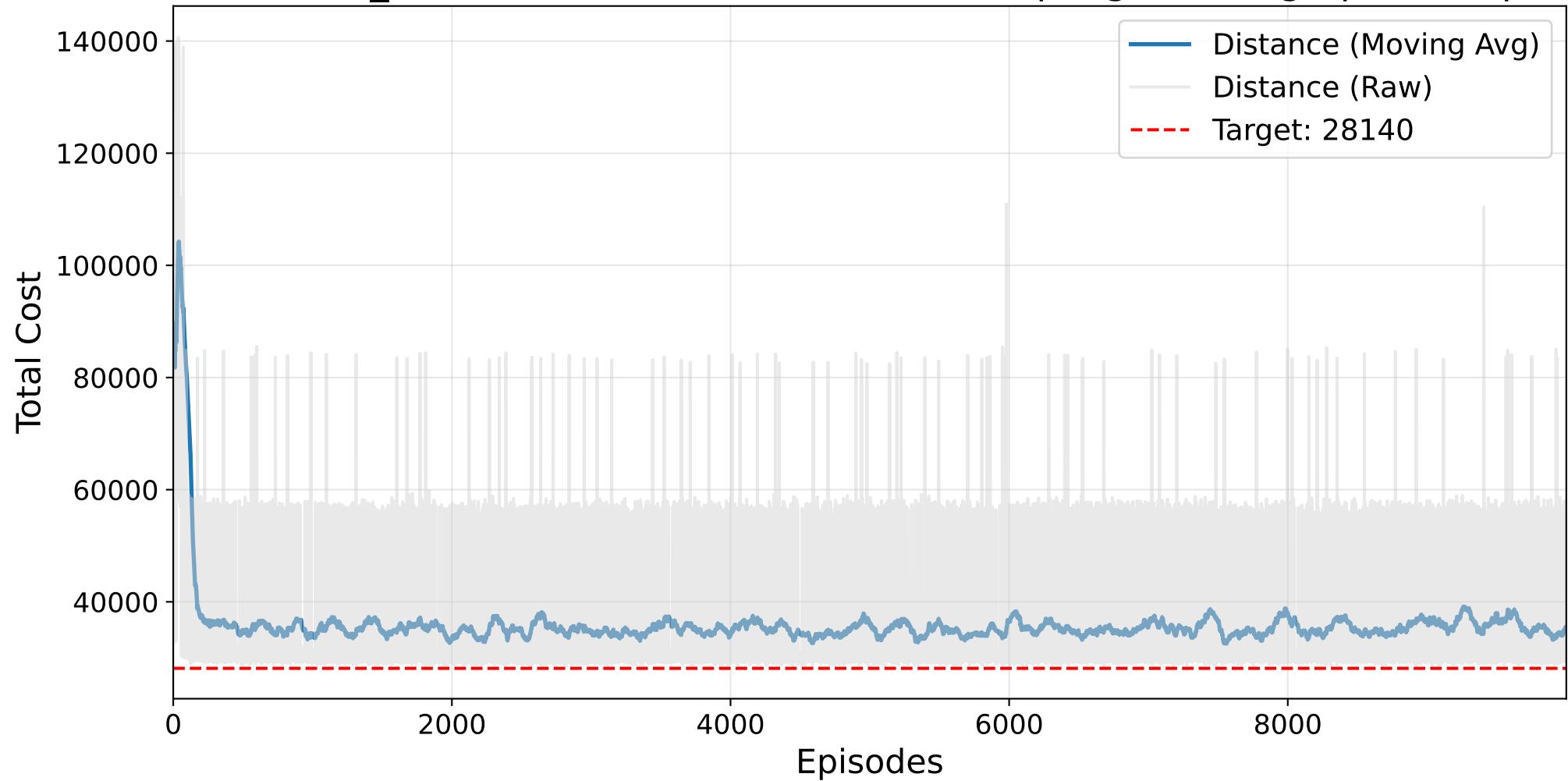
Final NO_MASK Masked AutoRL-SOP (Resampling) Training - p43.1.sop
